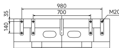
Robot Top View Fixed Platen
