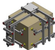
Crate Gripper
